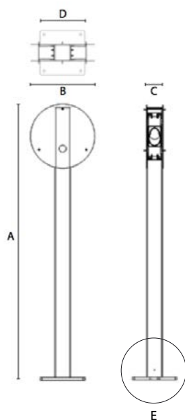
Fig. 1 - Freestanding mount shown with Pod Point solo unit mounted on it.
